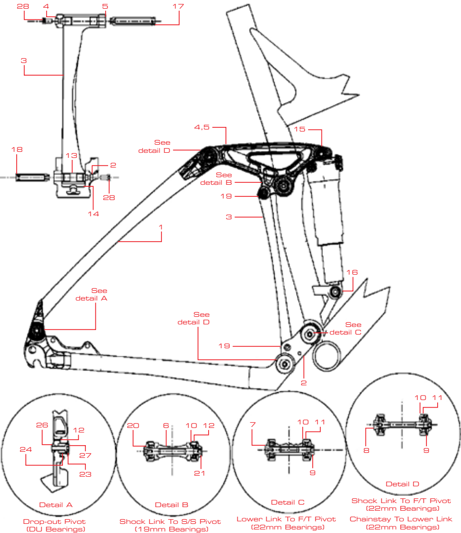
Virtue Alloy/Alloy Series Parts Illustration.
